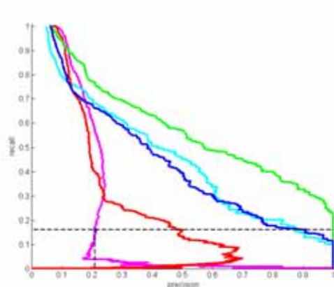
(b) Leaving, Camera 2 sequences (TM-FR)
