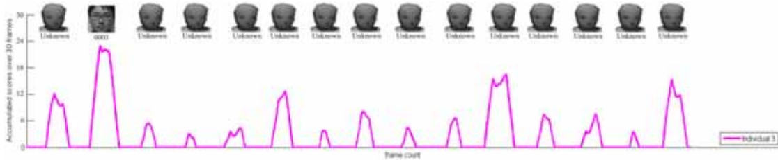
(a) Accumulated scores when face captures are matched against the reference ROI of ID 03.
