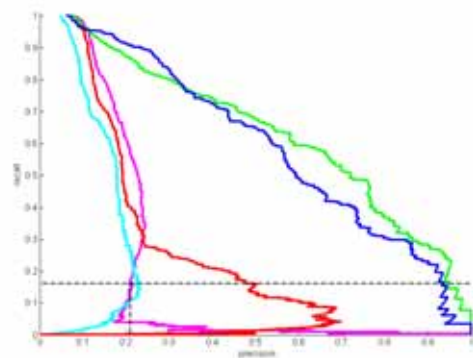
(d) Leaving, Camera 2 sequences (TM-FR with self-update)
