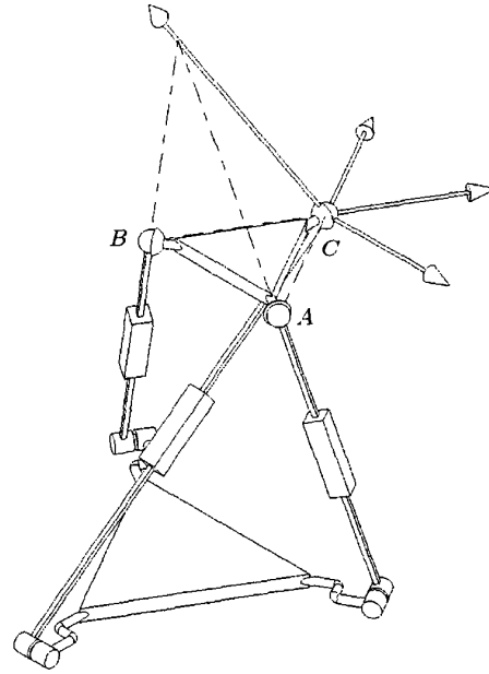
Figure 4: A constraint singularity of a 3-RPS mechanism
