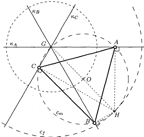
Figure 5: Constraint singularities of a 3-RPS mechanism
