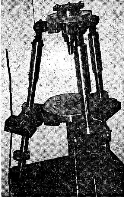
Figure 1: The 3-UPU mechanism at SNU in a singular configuration (courtesy of Prof. Frank Park)
