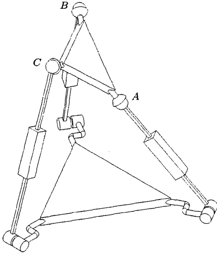
Figure 3: An RO-type singularity of a 3-RPS mechanism
