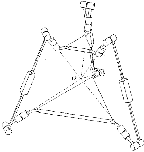
Figure 2: A 3- UPU wrist in a constraint singularity
