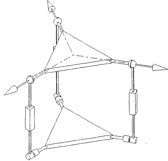
Figure 6: A 3-RPS PM in a constraint singularity
