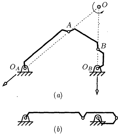
Figure 7: A flattened four-bar mechanism in (a) a nonsingular configuration and (b) a constraint singularity
