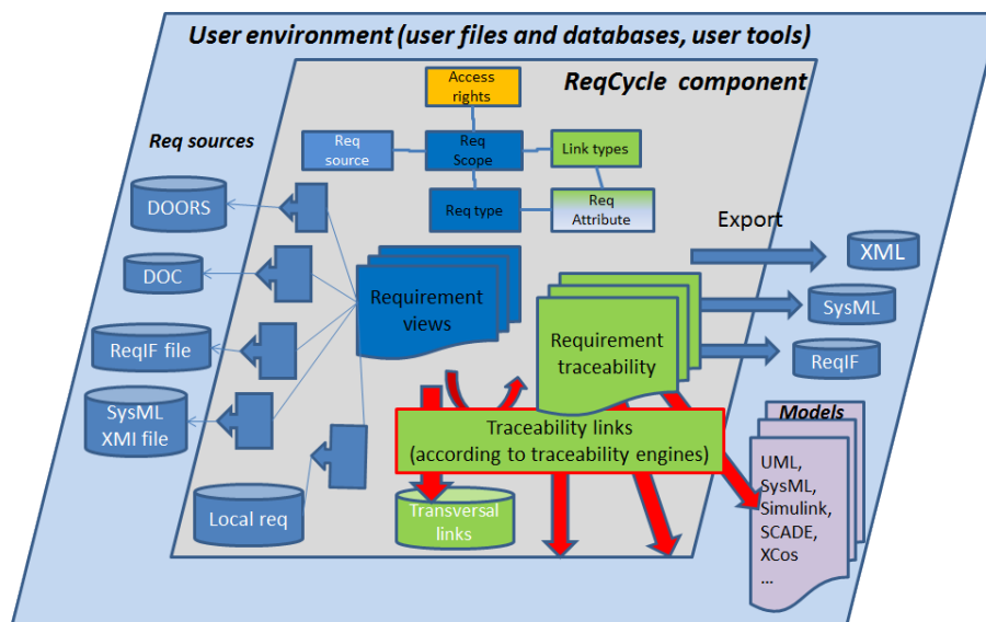
Figure 3. Polarsys ReqCycle Requirements Management Component
